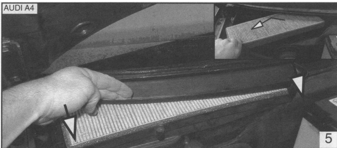
Step 5: Remove water-catch trim piece by pulling it straight out towards the front of the car. Two metal clips hold it in, one on each side of the trim piece. Remove old dust/pollen filter. Clean out any debris from the blower-fan area with a vacuum.
