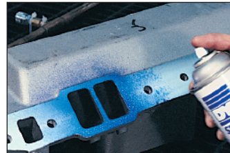
The spray Dykem is again used on the intake manifold.
