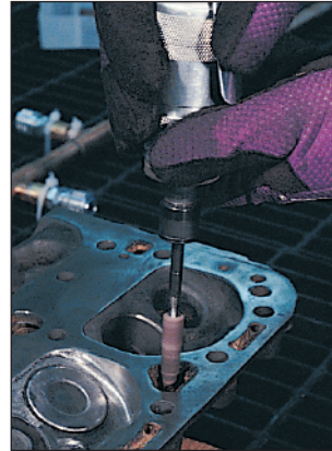
Most heads will have a lot of casting flash in the water crossovers. Use a small cartridge roll to remove that flash.
