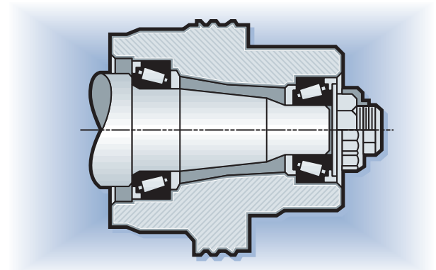
Figure 1: Passenger car non-driven wheel setting method
