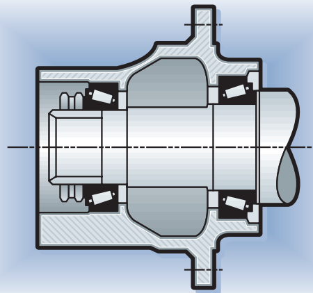
Figure 2: Independent suspension rear axle setting method
